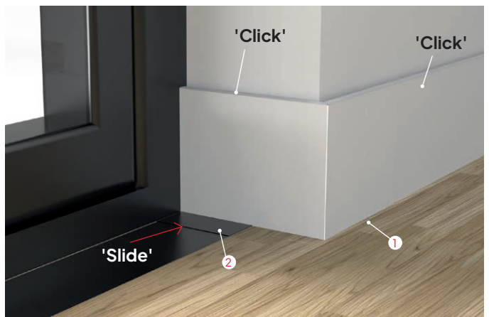
Use a special Threshold cover to conceal the plasterwork and slide an open ended cover at the floor mounted intersection. TOP TIP: Silicone seal between covers and door frame.
