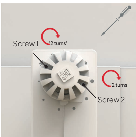
Position the holes in knob as shown to access 2 fixing screws for TRV controls.
