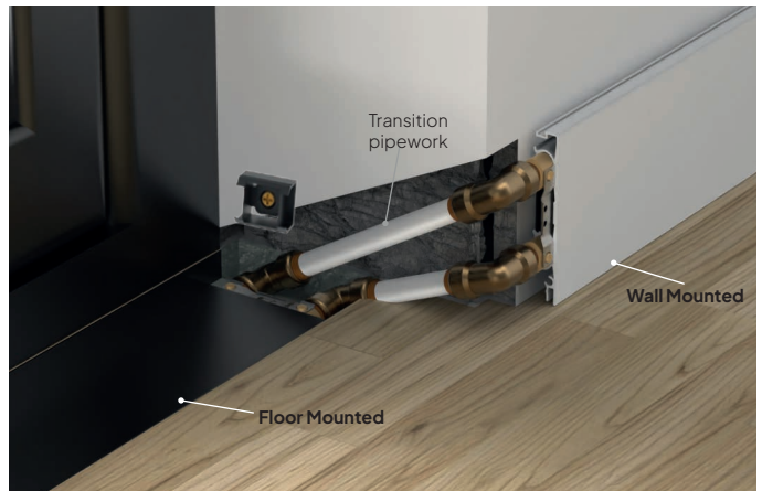
Install the floor and wall mounted Skirting, both connected via the transition pipes (Not Supplied).
