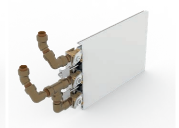
Pipes dropping from above (Solid wall)
