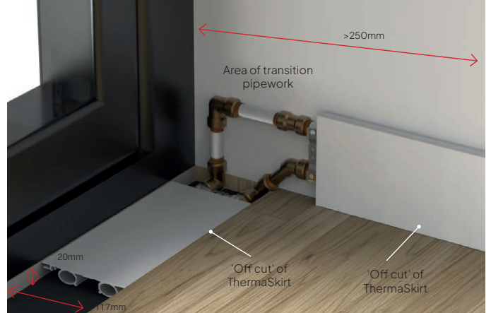
Using offcuts and connectors, Create a transition model as shown. Sections of pipes must be used for the connection (Not Supplied).
