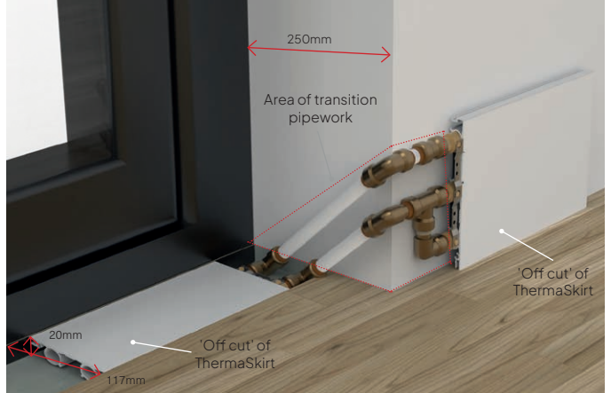
Place an offcut of skirting into the channel and wall, creating a transition jig. Mark the area of angle and profiles of the transition pipes.
