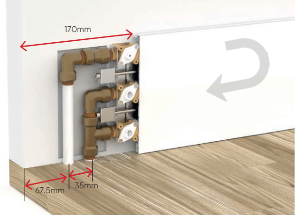
Clockwise Manual TRV
