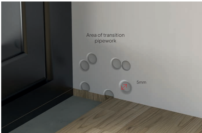
Relieve the wall 5mm as shown for the tectites to sit flush to the skirting, this ensures the flawless fitting of covers.
