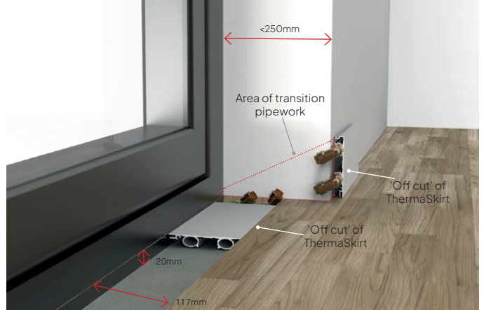
Place an offcut of skirting into the channel and wall, creating a transition jig. Mark the area of angel and profiles of the transition pipes.
