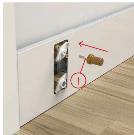
Insert the wax element into the TRV valve before fitting the TRV knob. Do not forget the white spacer!
