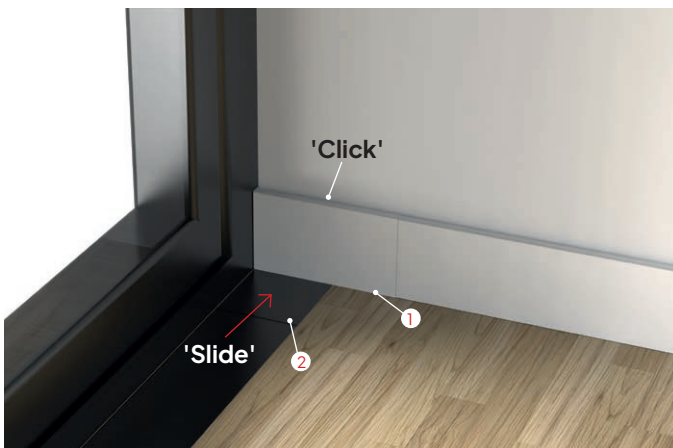
Use a close ended Threshold cover to conceal the plasterwork and slide an open ended cover at the floor mounted intersection.
