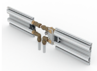
Pipes through floor
